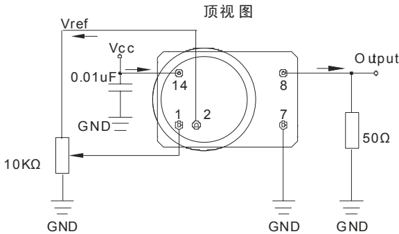
恒温晶振测试线路图(Sinewave,50Ω)
