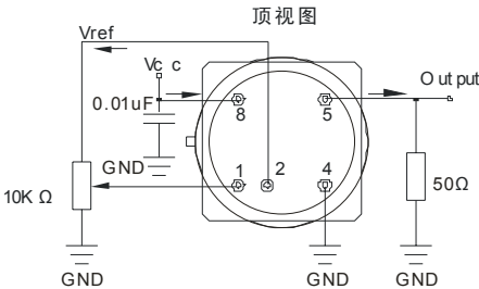
恒温晶振测试线路图(Sinewave,50Ω)
