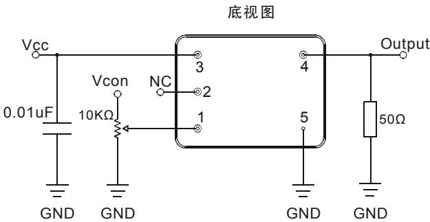
恒温晶振测试线路图(Sinewave,50Ω)
