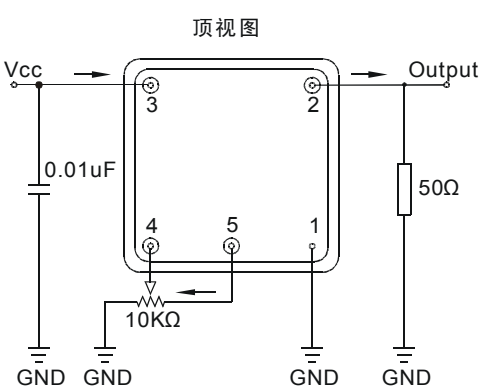
恒温晶振测试线路图(Sinewave,50Ω)
