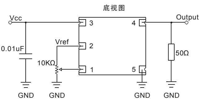
恒温晶振测试线路图(Sinewave,50Ω)
